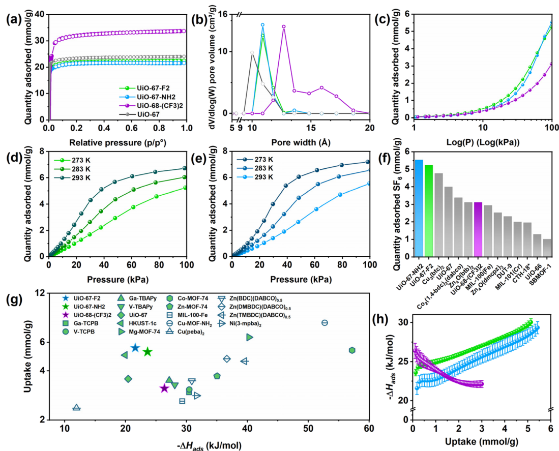
Fig. 2 (a) Nitrogen sorption isotherms recorded at -196^{\circ}\text{C} . Adsorption and desorption branches of the isotherms are depicted using filled and hollow circles, respectively. (b) DFT pore size distributions, (c) \text{SF}_6 adsorption isotherms recorded at 20^{\circ}\text{C} , (d) \text{SF}_6 adsorption isotherms for UiO-67- \text{F}_2 recorded at 0 – 20^{\circ}\text{C} , (e) \text{SF}_6 adsorption isotherms for UiO-67- \text{NH}_2 recorded at 0 – 20^{\circ}\text{C} , and (f) comparison of the \text{SF}_6 adsorption capacity at 100\text{ kPa} of various MOF sorbents, measured at 20^{\circ}\text{C} . 35–42 (g) Comparison of the \text{SF}_6 adsorption capacity at 100\text{ kPa} and enthalpies of \text{SF}_6 adsorption of various published MOF sorbents, measured at 20^{\circ}\text{C} . 35–42 (h) Isosteric enthalpies of \text{SF}_6 adsorption, error bars from each point in the linear adaptation to the isosteres.
