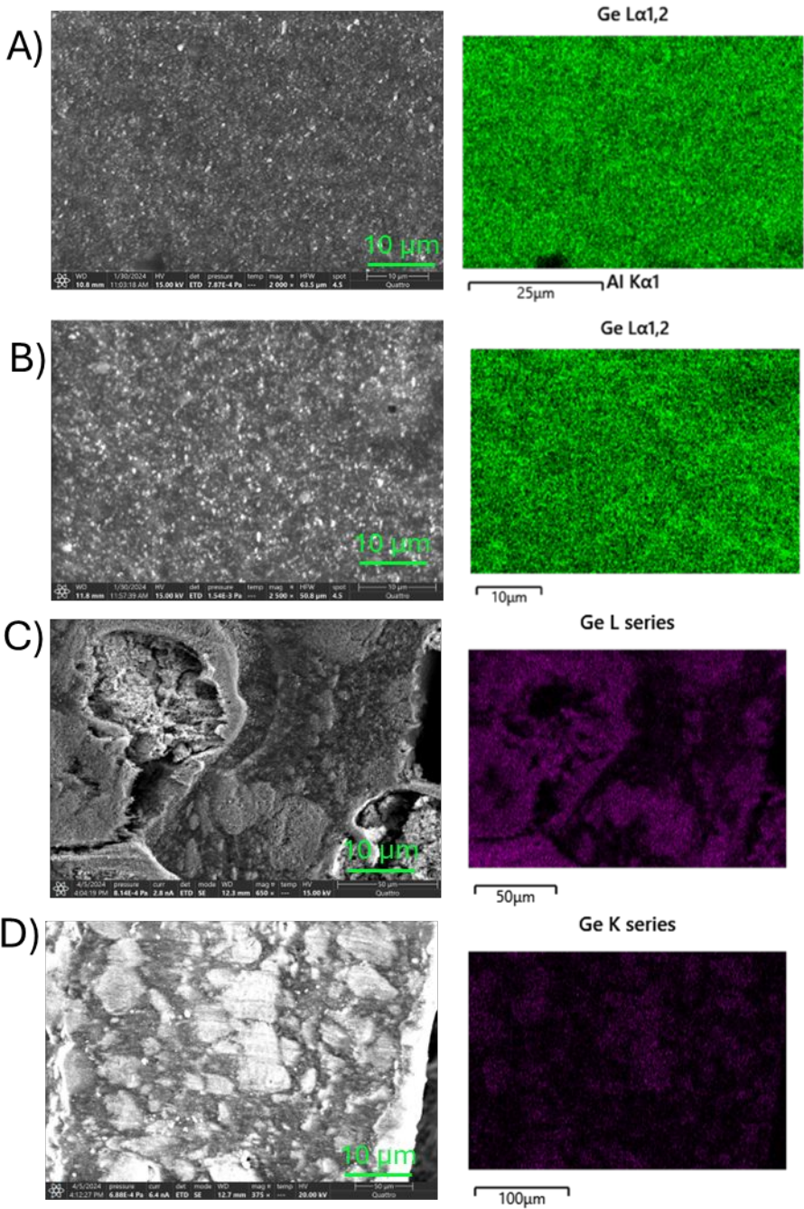
Figure 2: SEM images of sliced PEO-LAGP electrolytes with germanium mapping via EDX. A) PEO(LiTFSI)-LAGP MP, B) PEO(LiBOB)-LAGP MP, C) PEO(LiTFSI)-LAGP SC, D) PEO(LiBOB)-LAGP SC. All images represent cross sections of the hybrid electrolytes. Samples were sliced with a blade following cooling with dry ice. The images were acquired with an accelerating voltage of 15 kV and magnifications ranging from 670 to 2300x.
