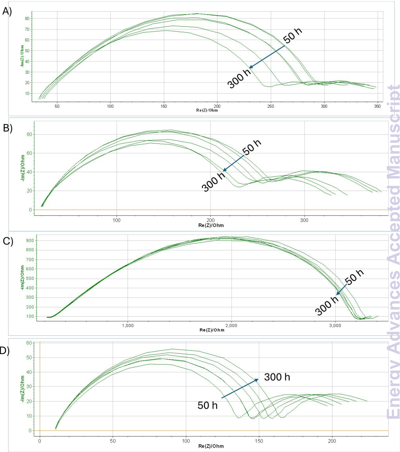
Figure 6: Impedance spectra of PEO(LiBOB)-LAGP following cycling in Li-Li symmetric cells at 60 °C for a period spanning 50 to 300 hours. The spectra presented in A) correspond to the MP
