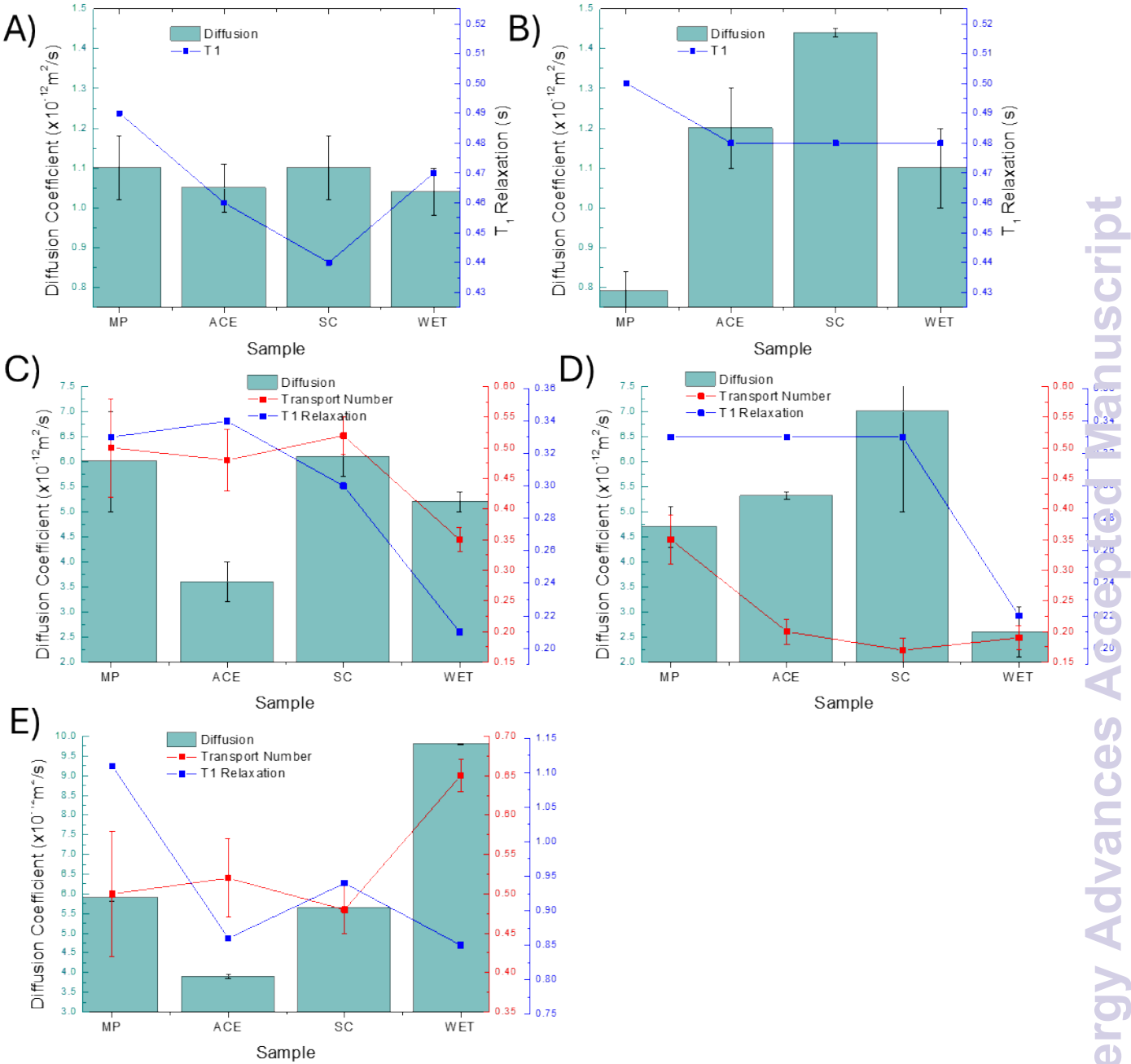
Figure 4: Ion mobility at 60 °C as determined by solid-state NMR spectroscopy. A) and B) represent proton mobility in PEO(LiTFSI)-LAGP and PEO(LiBOB)-LAGP samples respectively while C) and D) represent lithium mobility in PEO(LiTFSI)-LAGP and PEO(LiBOB)-LAGP respectively. E) represents fluorine mobility in PEO(LiTFSI)-LAGP. All spectra were acquired at 9.4 T with 5 kHz MAS. Lithium transport numbers for the LiBOB-containing samples were determined electrochemically using the Bruce-Vincent method.
