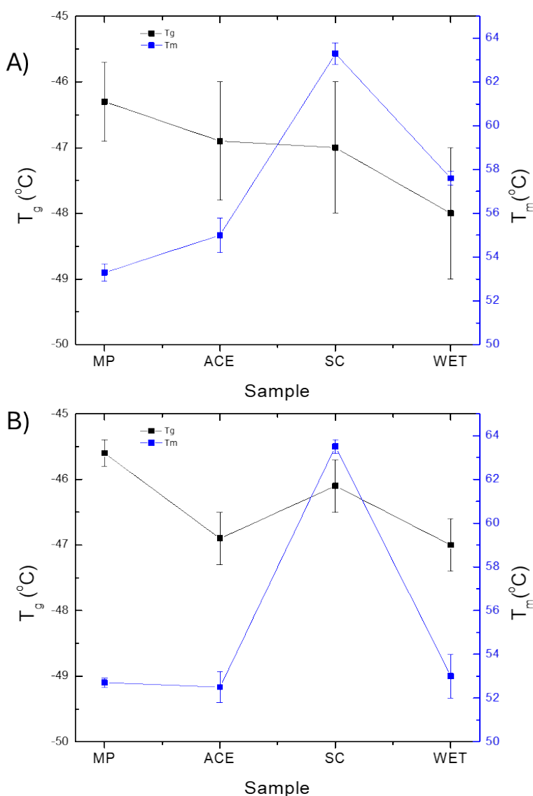
Figure 3: T_g and T_m of PEO(LiTFSI)-LAGP (A) and PEO(LiBOB)-LAGP (B) as determined by DSC. Samples were heated from -50 to 150 °C at a rate of 10 °C/min during data collection.
