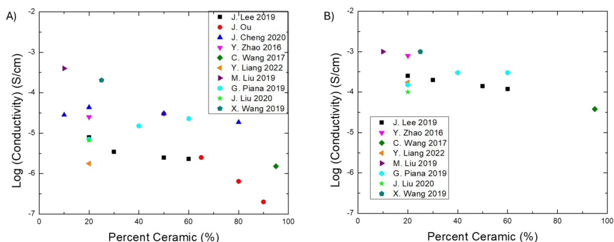
Figure 1: Ionic conductivity as a function of LAGP content for previously published examples of PEO-LAGP hybrid electrolytes at A) 30 °C and B) 60 °C.
