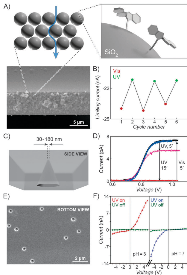
Fig. 19 Light-controlled transport through porous materials. (A and B) Effect of irradiation on the flux of a charged redox probe through densely packed, spirropyran-functionalised colloidal spheres. (C) Schematic representation of a conical nanopore with spirropyran-functionalised interior. (D) Light-controlled transport through a conical nanopore. Formation of the positively charged \text{MCH}^+ inhibits the flux of a positively charged probe. (E) SEM image showing multiple spirropyran-functionalised nanopores. (F) Ionic current rectification modulated by pH and light. [Adapted with permission from ref. 377 (Copyright 2010 Springer) (A and B), ref. 378 (Copyright 2006 Royal Society of Chemistry) (D) and ref. 379 (Copyright 2012 Wiley-VCH) (E and F)].
