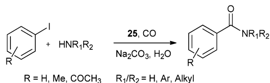
Scheme 31 Reagents and conditions: aryl iodide (1 mmol), amine (2 mmol), Na_2CO_3 (2 mmol), 25 (50 mg, 14.2\ \mu mol ), water (10 mL), CO pressure (100 psi), temp. 100^\circ C , time 8 h.
