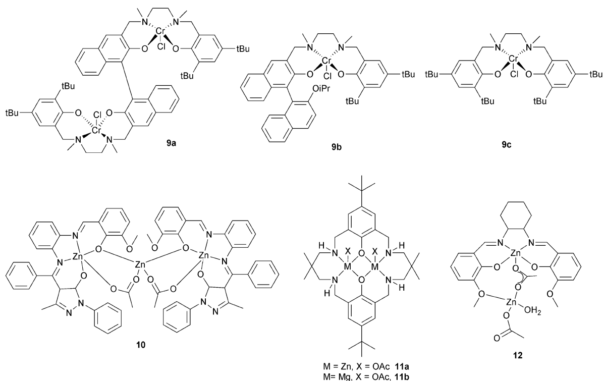
Fig. 7 Illustrates the structures of various bimetallic catalysts.
