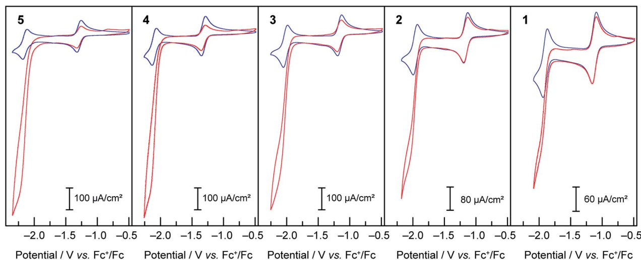
Fig. 6 Cyclic voltammograms under Ar (— blue) and \text{CO}_2 (— red) at 50 \text{ mV s}^{-1} of 1 \text{ mM} solutions of compounds 1–5 in DMF/ \text{H}_2\text{O} (95 : 5), TBAPF 6 0.1 \text{ M} .
