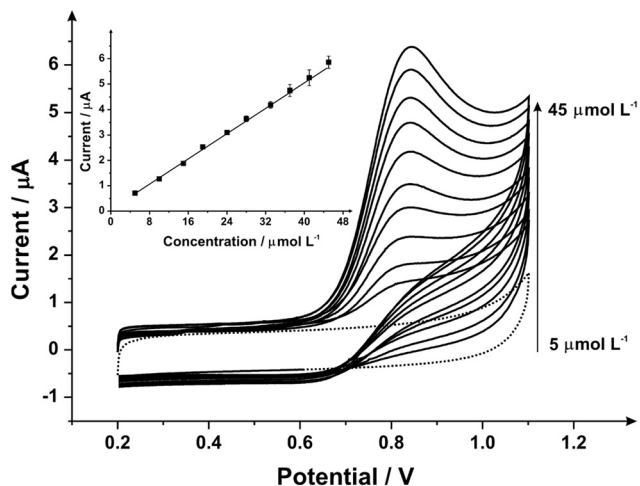
Fig. 7 Cyclic voltammograms obtained from additions of sodium nitrite ( 5\text{--}45\ \mu\text{mol L}^{-1} ) into pH 7 PB using a 1 minute mechanically activated/polished SPE with diamond slurry using the same SPE throughout the experimentation (scan rate: 100\ \text{mV s}^{-1} vs. SCE); the dotted line represents the blank (no sodium nitrite) response. Inset: analysis of the voltammetric peak heights as a function of concentration.
