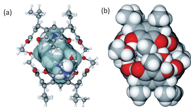
Fig. 2 Dimeric capsule, (\text{TDAC})^{2+} @ 1 \cdot \text{H}_2\text{O} \cdot \text{MeOH}_2 shown in (a) as ball and stick with the calculated cavity in transparent grey colour and the guest (\text{TDAC})^{2+} as CPK to illustrate the very tight encapsulation and (b) as the CPK model.
