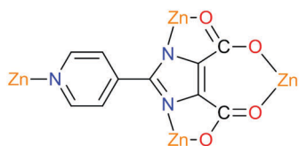
Fig. 12 Section of the structure of [\text{Zn}_2(\text{pidc})(\text{H}_2\text{O})\text{Cl}]_n . 78
