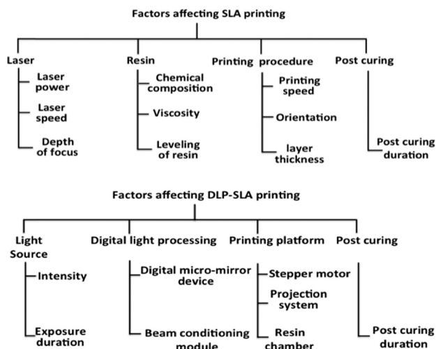
Fig. 8 Parameters affecting laser and DLP-SLA print process.
