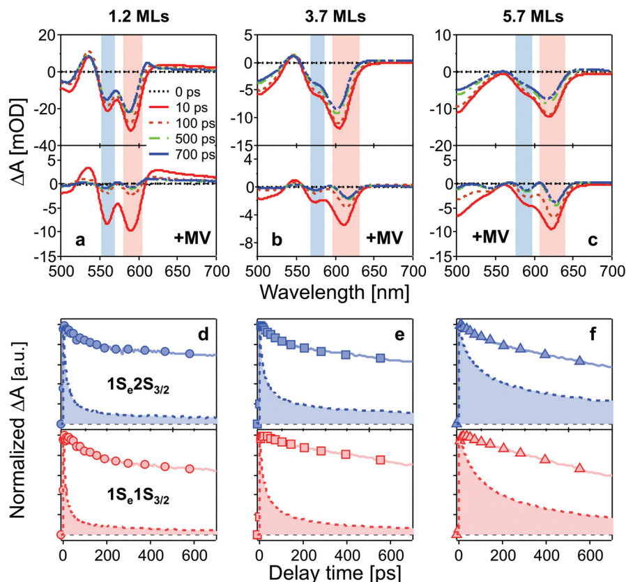
Fig. 2 (a–c): TA spectra of CdSe/CdS QDs (top) and QD- MV^{2+} complexes (bottom) at different delay times after 400 nm excitation. Bleaching peaks are assigned to different exciton states indicated by color blocks in each panel (red: 1S_e1S_{3/2} ; blue: 1S_e2S_{3/2} ). (d–f): normalized bleaching kinetics of 1S_e1S_{3/2} (bottom, red) and 1S_e2S_{3/2} (top, blue) state in three batches of QDs (solid lines) and QD- MV^{2+} complexes (dashed lines and filled areas) within 700 ps. The concentrations of all QD solutions were 3 \mu M and the number of added MV^{2+} per QD was 10 for all QD- MV^{2+} samples. The excitation power was kept low for all measurements in order to avoid multi-exciton effect (see ESI†).
