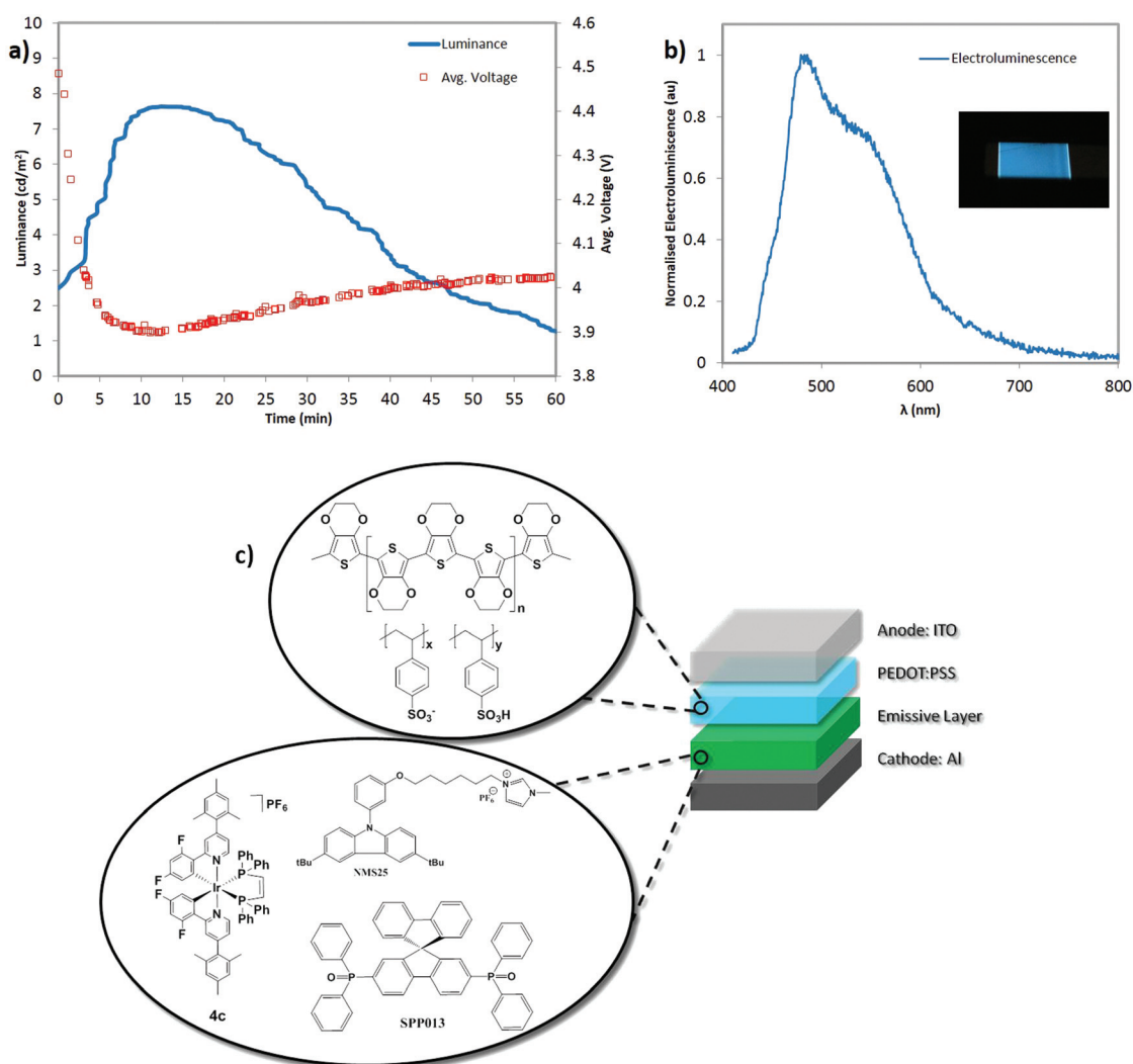
Fig. 5 (a) Luminance (solid blue line) and average voltage (open red squares) for ITO/PEDOT:PSS/active layer/Al (active layer = 1 : 1 by mass of NMS25 : SPPO13 with 10 wt% of 4c) with a pulsed driving regime (block-wave pulsed current; 1000 Hz; 50% duty cycle; average density 100 A m -2 ). (b) Electroluminescence spectrum with inset photo of LEEC. (c) Schematic representation of the LEEC architecture.
