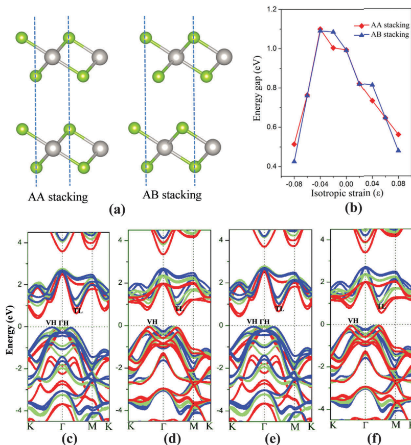
Fig. 5 (a) Atomic structure of two kinds of PtSe 2 bilayers. (b) Band gap of PtSe 2 bilayers versus isotropic strain. Computed band structure of AA stacking bilayers under (c) \varepsilon = -8 to 0%, (d) \varepsilon = 0-8\% and AB stacking bilayers under (e) \varepsilon = -8 to 0%, (f) \varepsilon = 0-8\% . The bands with different colors represent the band structures under various strain values, i.e. , blue ( \varepsilon = 0\% ), green ( \varepsilon = \pm 4\% ) and red ( \varepsilon = \pm 8\% ). The Fermi level is located at 0 eV.
