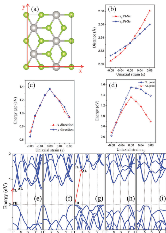
Fig. 4 (a) A rectangle supercell of monolayer PtSe 2 where x - and y -directions are defined. (b and c) Pt–Se bond length and band gap of monolayer PtSe 2 versus uniaxial strain, respectively. (d) The energy of the AL and \Gamma L points with respect to the Fermi level versus \varepsilon_y . Computed band structure of monolayer PtSe 2 with strain values of (e) \varepsilon_y = -8\% , (f) \varepsilon_x = -8\% , (g) \varepsilon = 0\% , (h) \varepsilon_x = 8\% and (i) \varepsilon_y = 8\% . The Fermi level is set to be 0 eV.
