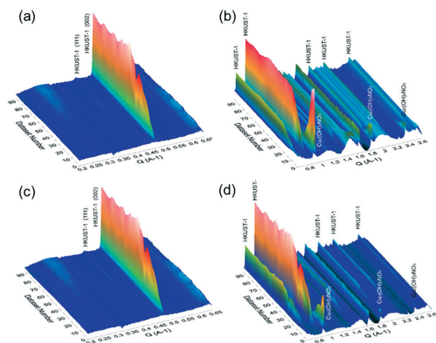
Fig. 4 Time series of radially averaged SAXS (a and c) and WAXS (b and d) data. The nucleation and growth of \text{Fe}_3\text{O}_4@ \text{HKUST-1} (a and b) and HKUST-1 (c and d) at room temperature is observed when the alcoholic solution containing \text{H}_3\text{BTC} is added to the solution containing Cu-based precursors. Dataset number corresponds to SAXS/WAXS images were collected every 3.15 s. The ligand was injected at t = 30 \text{ s} (dataset 10).
