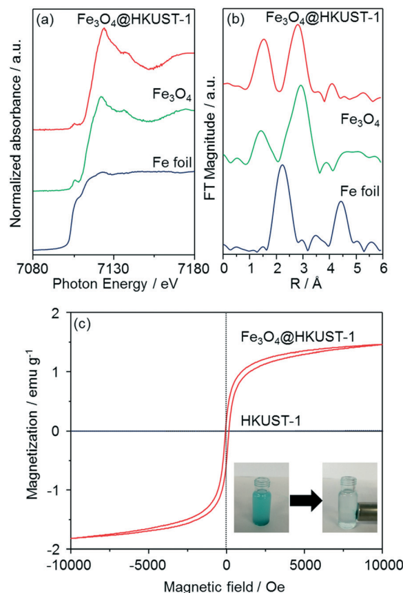
Fig. 5 Fe K-edge (a) XANES and (b) FT-EXAFS spectra of \text{Fe}_3\text{O}_4 , \text{Fe}_3\text{O}_4@ \text{HKUST-1} and Fe metallic foil. (c) Magnetization curves of \text{Fe}_3\text{O}_4@ \text{HKUST-1} and HKUST-1, and photographs of \text{Fe}_3\text{O}_4@ \text{HKUST-1} collected by a magnet. The magnetization measurements were performed at 300 K.
