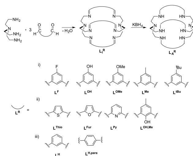
Scheme 1 Azacryptands L A R and imines L 1 R with different linker molecules L R . The linkers are arranged according to their (i) different steric bulks on the central benzyl unit, (ii) capability to directly alter the electron density within the azacryptand cavity and (iii) different cage sizes. 5,14,15,17,20
