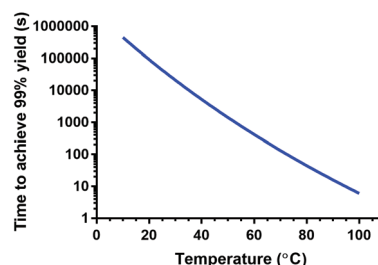
Fig. 6 Prediction of time needed to achieve 99% yield for [¹⁷⁷Lu]Lu-DOTA-TATE in a setup with optimal heat and mass transfer. The graph was calculated using the Arrhenius parameters obtained in this study.
