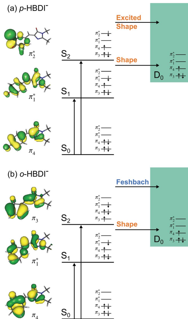
Fig. 6 Energy level diagram of (a) p -HB \text{DI}^- and (b) o -HB \text{DI}^- in which possible excitations and subsequent detachment processes are indicated (note that it is only the vibrationally excited states of S_1 lying in the D_0 continuum that have shape resonance character). S_1 and S_2 refer to the first two excited states selected in Table 2. The HOMO is \pi_4 and the LUMO is \pi_1^* . Alongside are the Hartree–Fock molecular orbitals that are involved in the excitations. For op -DH \text{BDI}^- , a similar scheme applies as for p -HB \text{DI}^- except the excited state resonance is S_3 (Table 2).
