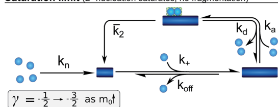
Fig. 3 A schematic depiction of the reaction network for the aggregation of A \beta 42. The general network (top), the special case when both fragmentation and unsaturated secondary nucleation are important (centre), resulting in a parallel network, and the special case where saturation of secondary nucleation is important (bottom) but fragmentation is negligible. The ranges of approximate scaling exponents for each of these cases as the monomer concentration increases are given below each scheme. The rate constants given denote primary nucleation ( k_n ), elongation ( k_+ ), depolymerisation ( k_{off} ), fragmentation ( k_- ), single-step secondary nucleation ( k_2 ), and the rates associated with multi-step secondary nucleation: the monomer attachment ( k_a ) and detachment rate constants ( k_d ), and the nucleus conversion/detachment rate constant ( k_2 ).
