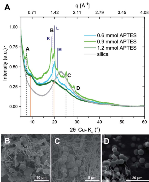
Fig. 6 PI6/SiO _2 prepared from PMA, HMDA, APTES and TEOS. (A) Diffractograms of the hybrids prepared at different n_{\text{APTES}} , and diffractogram of hydrothermally synthesized SiO _2 for comparison (grey). (B)–(D) SEM images of the corresponding hybrids at n_{\text{APTES}} = 0.6 mmol (B), n_{\text{APTES}} = 0.9 mmol, and n_{\text{APTES}} = 1.2 mmol.
