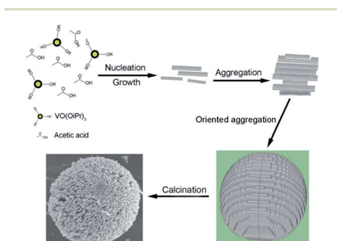
Fig. 11 Schematic of the formation of 3D porous \text{V}_2\text{O}_5 hierarchical microspheres. 103
