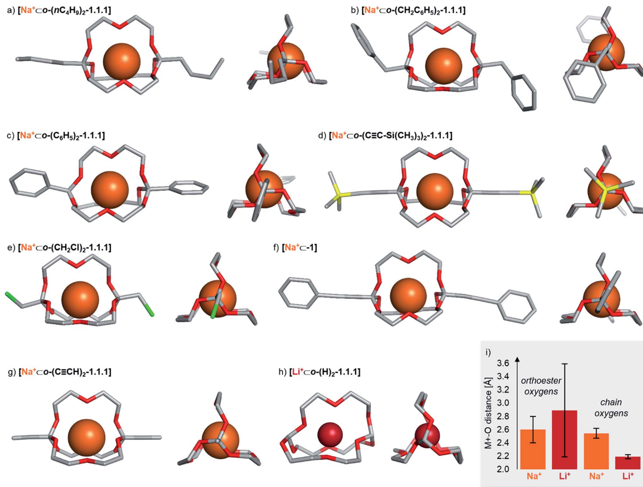
Chart 1 Solid-state structures of eight orthoester cryptands. Single crystals were obtained by the layering method (hexane/chloroform). Hydrogen atoms, anions, solvent and disorder (where applicable) are omitted for clarity. Metal ions are displayed at 100% of effective ionic radius. 27 (a) Crystal system: triclinic. Na–O distance (orthoester oxygen): 2.45–2.92 Å. Na–O distance (chain oxygen): 2.48–2.53 Å. (b) Crystal system: monoclinic. Na–O distance (orthoester oxygen): 2.47–2.76 Å. Na–O distance (chain oxygen): 2.51–2.57 Å. (c) Crystal system: orthorhombic. Na–O distance (orthoester oxygen): 2.32–3.53 Å. Na–O distance (chain oxygen): 2.37–2.46 Å. (d) Crystal system: triclinic. Na–O distance (orthoester oxygen): 2.48–2.59 Å. Na–O distance (chain oxygen): 2.54–2.67 Å. (e) Crystal system: monoclinic. Na–O distance (orthoester oxygen): 2.47–2.89 Å. Na–O distance (chain oxygen): 2.48–2.57 Å. (f) Crystal system: triclinic. Na–O distance (orthoester oxygen): 2.43–2.69 Å. Na–O distance (chain oxygen): 2.56–2.61 Å. (g) Crystal system: triclinic. Na–O distance (orthoester oxygen): 2.46–2.66 Å. Na–O distance (chain oxygen): 2.53–2.67 Å. (h) Crystal system: orthorhombic. Li–O distance (orthoester oxygen): 1.96–3.67 Å. Li–O distance (chain oxygen): 2.16–2.23 Å. (i) Comparison of average Na–O distance of all sodium-based solid-state structures with average Li–O distance in [\text{Li}^+ \subset \text{o}-(\text{H})_2-1.1.1] , including standard deviation. For further details, see ESI.†
