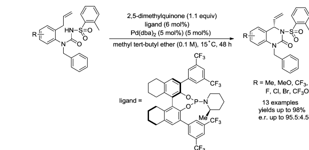
Scheme 26 Synthesis of chiral hydropyrimidinones.
