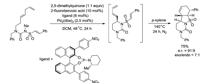
Scheme 27 Synthesis of a chiral polycyclic heterocycle.
