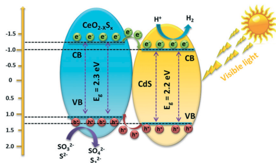
Scheme 2 Schematic diagram of the proposed charge carrier transfer and \text{H}_2 evolution mechanism over the \text{CeO}_{2-x}\text{S}_x @CdS photocatalyst under visible-light irradiation.
