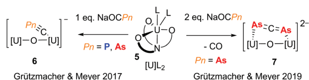
Fig. 2 Reactivity of a uranium(III) complex with phosphaaethynolate and arsaethynolate.
