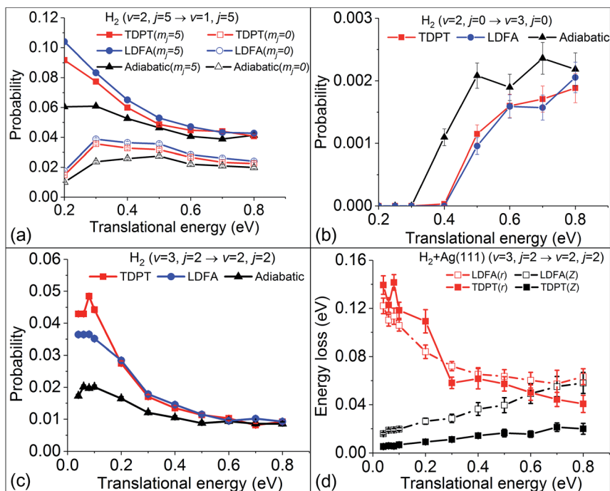
Fig. 5 (a) Vibrational state-to-state deexcitation probabilities from \text{H}_2 ( v = 2, j = 5 ) to \text{H}_2 ( v = 1, j = 5 ) for rotationally excited initial conditions as predicted with MD, MDEF(LDFA), and MDEF(TDPT). (b) Vibrational excitation probabilities upon scattering. (c) Vibrational deexcitation probability from \text{H}_2 ( v = 3, j = 2 ) to \text{H}_2 ( v = 2, j = 2 ). (d) Energy loss during vibrational deexcitation from \text{H}_2 ( v = 3, j = 2 ) to \text{H}_2 ( v = 2, j = 2 ).
