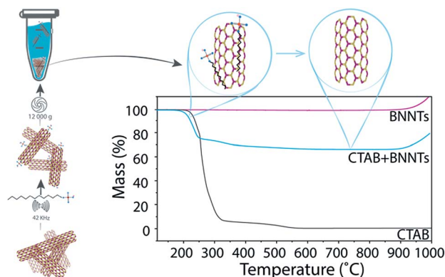
Fig. 1 Schematic demonstrating how the experiment is performed (left) and TGA profiles of BNNTs, CTAB, and a BNNT–CTAB pellet (right). Samples containing CTAB experience a drop in mass from 200–400 °C due to burning of the organic surfactant. BNNTs are oxidized above 900 °C, resulting in a rapid increase in mass. The minimum mass% (at 700 °C) is used to determine the mass of BNNTs in the sample.
