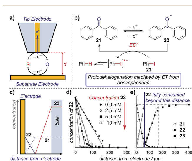
Fig. 22 (a) Schematic of an SECM set-up, where the distance ( d ) between the substrate and tip electrodes can be changed to measure concentrations in solution. The concentration profile of species in the mediated reduction of iodobenzene (b), measured by Amatore et al. using SECM. (c) Schematic of concentration profiles. (d) Concentration profile of 22 with varying equivalents of 23, measured by changing the distance ( d ) between the two electrodes. (e) Comparative concentration profile of various species in solution. (c–e) Adapted with permission from ref. 75. Copyright 2001 John Wiley and Sons.
