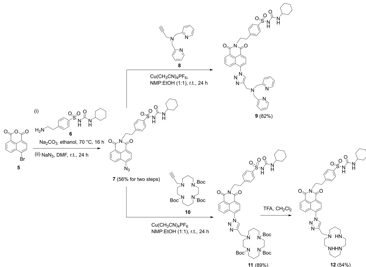
Scheme 1 The successful synthetic route to probes 9 and 12 incorporating cyclohexyl sulfonamide as the ER targeting unit.
