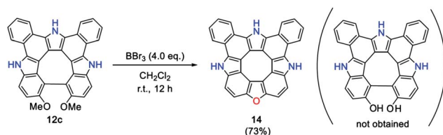
Scheme 2 Synthesis of triazaaza[8]circulene 14 .
