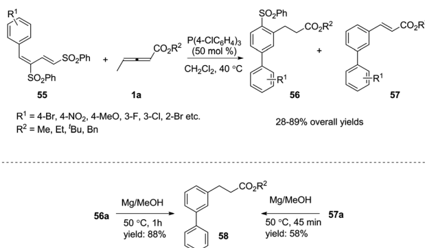
Scheme 17 Phosphine-catalysed (2+4) benzannulation reaction.
