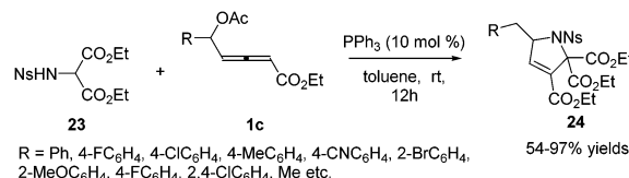
Scheme 7 Phosphine-catalysed (3+2) annulation of \delta -acetoxy allenoates with 2-sulfonamidomalonate.
