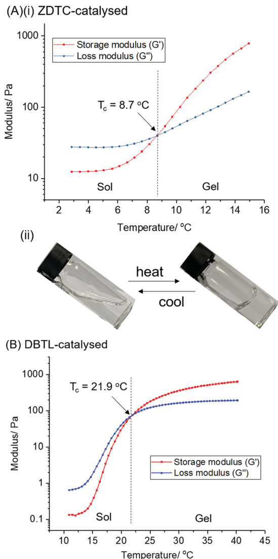
Fig. 2 Oscillatory temperature sweep showing the changes in storage ( G' ) and loss modulus ( G'' ) as a function of temperature, as well as the gelation temperature of 10 wt% PU catalysed by (A) ZDTC and (B) DBTL. Figure (A)(ii) shows the reversible sol–gel transition of a transparent 10 wt/v% solution of ZDTC-catalysed PU in water.
