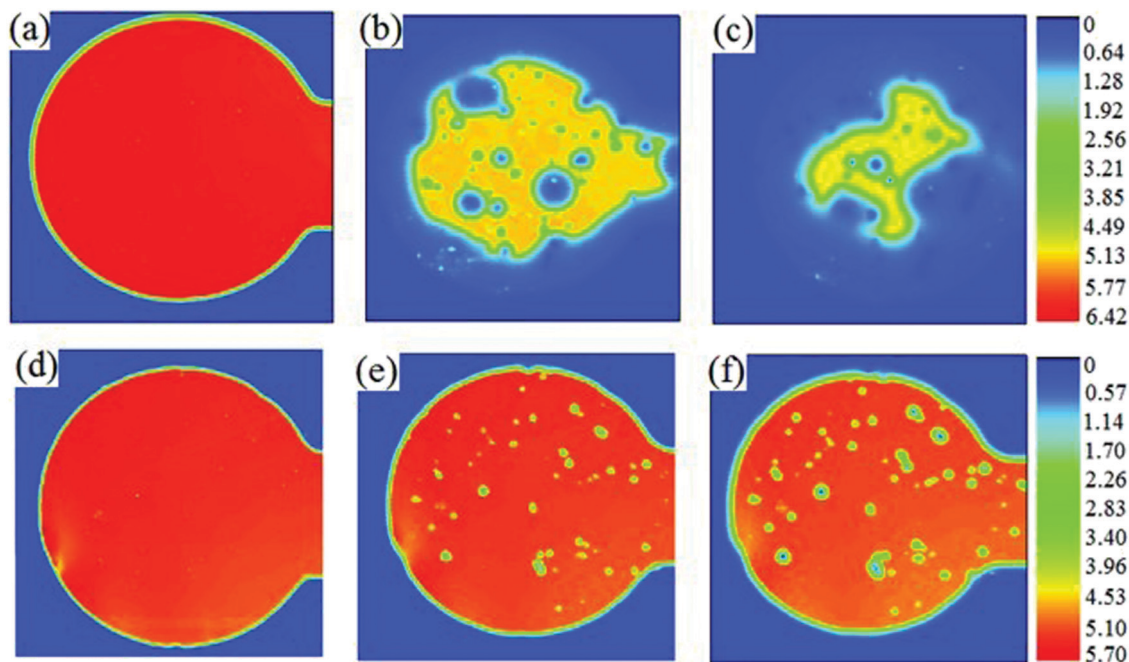
Fig. 5 Laser beam induced photocurrent images of the devices exposed to ambient air: (a and d) 0 days; (b and e) 4 days and (c and f) 8 days. The hole-transport layer was PEDOT:PSS (a–c) or \text{MoO}_3 -PEDOT:PSS (d–f). The colour scale represents the photocurrent. Reproduced with permission. 41 Copyright 2013, WILEY-VCH Verlag GmbH & Co. KGaA, Weinheim.
