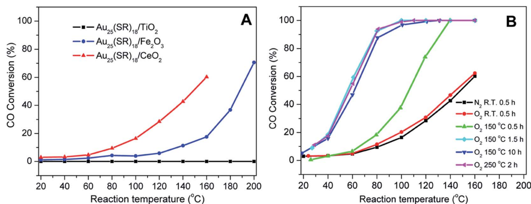
Fig. 3 Activation of Au 25 (SR) 18 clusters over different metal oxides for CO oxidation. (A) CO activity over different metal oxides as a function of temperature for unactivated clusters, and (B) CO activity on ceria supports under different activation conditions. Reprinted with permission from ref. 49. Copyright 2012, American Chemical Society.
