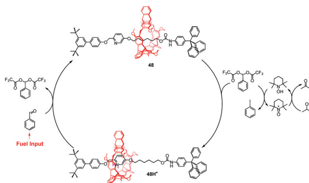
Fig. 44 Switchable motion of the [2]rotaxane powered by step-by-step reaction.
