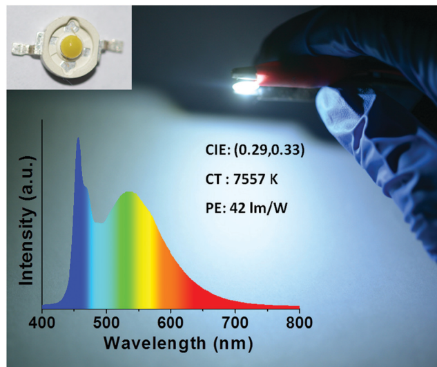
Fig. 6 Photograph of a CD-based working LED prototype utilizing a \text{CDs@g-C}_3\text{N}_4 composite with 1 wt% CDs as a phosphor, and its emission spectra with the related characteristics. CIE: CIE color coordinates, CT: color temperature, PE: power efficiency.
