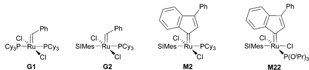
Fig. 1 Commercial Type 1 initiators used for the polymerisation of DCPD. \text{PCy}_3 = tricyclohexylphosphine; SIMes = 1,3-dimesitylimidazolidin-2-ylidene.
