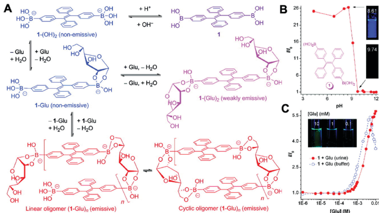
Fig. 10 (A) Proposed mechanism for the process of glucose-specific sensing by AIE-active sensor 1 . (B) Change in the FL intensity ( I/I_0 ) of sensor 1 at 440 nm with pH values; I_0 is the FL intensity at pH 12.01. Inset: Photographs of the mixtures of 1 in the aqueous buffers at pH 8.6 and 9.7 taken under the illumination of a hand-held UV lamp ( \lambda_{ex} = 365 nm). (C) Changes in the FL intensity ( I/I_0 ) of 1 (50 \mu M) with glucose concentration in artificial urine (red circle) and carbonate buffer (blue circle). I_0 is the FL intensity in the absence of glucose. The inset in panel C shows photographs of mixtures of 1 (50 \mu M) in artificial urines containing different amounts of glucose taken under UV illumination. Adapted with permission from ref. 41. Copyright 2010 American Chemical Society.
