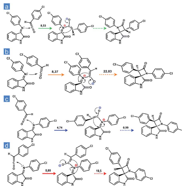
Fig. 4 Schiff base attacking a ketene carbonyl: (a) E -imine attacks from the hydrogen side; (b) E -imine attacks from the phenyl side; (c) Z -imine attacks from the hydrogen side; (d) Z -imine attacks from the phenyl side.
