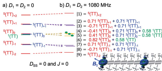
Fig. 4 Schematic representation of the sublevels of SCTP, as the weakly coupled multiexciton in (b) caused by the ZFS interactions ( D_1 = D_2 = 1080 MHz) of ^5 TIPS-Pn. The energy shifts in the SCTP levels in (b) are shown with respect to the levels in (a) with D_1 = D_2 = 0 in the presence of the external magnetic field (340 mT) for highly separated T + T ( D_{SS} = 0 and J = 0 ). The wavefunctions were computed for the field direction ( B_0 ) parallel to the out-of-plane axes of the aromatic rings.
