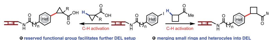
Fig. 1 Exploiting diversity of C–H activation in DELs.
