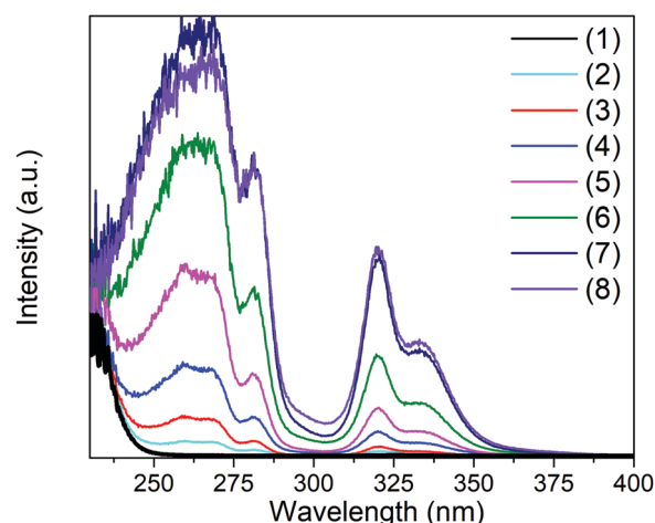
Fig. 2 Pseudo-absorbance obtained from Kubelka–Munk transformation of the diffuse reflectance data of Cs 2 NaInCl 6 :Sb 3+ for samples with various concentrations of Sb 3+ .
