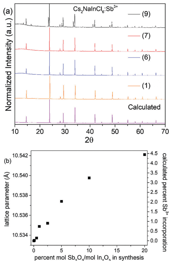
Fig. 1 (a) X-ray powder diffraction patterns of Cs 2 NaInCl 6 :Sb 3+ samples with varying amounts of Sb 2 O 3 added during synthesis, as well as the calculated diffraction pattern obtained from Rietveld refinement of the Sb-free host. The peaks in samples (1)–(8) can all be accounted for with a cubic double perovskite phase. The additional peaks in sample (9) arise from the presence of Cs 3 Sb 2 Cl 9 . (b) The lattice parameter for Cs 2 NaInCl 6 :Sb 3+ samples and calculated Sb 3+ incorporation percentages; the lattice constant error bars are smaller than the symbols.
