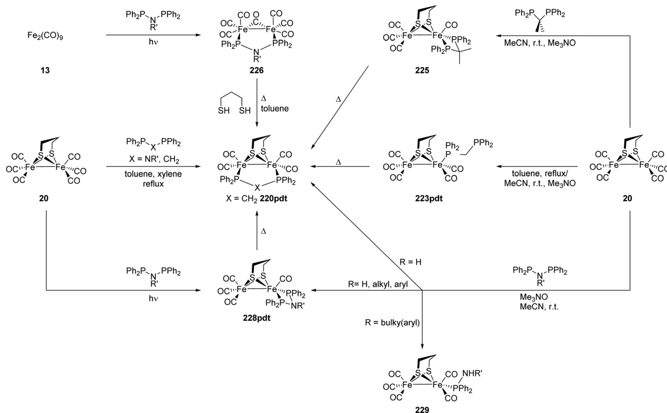
Fig. 65 Different synthetic pathways for the incorporation of dppe and derived ligands as well as PNP ligands into hydrogenase mimics.
