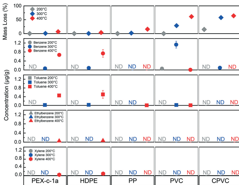
Fig. 3 Mean BTEX concentration after extracting each burned material at 200 °C, 300 °C, and 400 °C in water. CPVC. The error bars reflect the standard deviation of the measurements ( n = 3 ). If no error bars are visible, it indicates they were smaller than the symbol size. ND indicates the compound was not detected.
