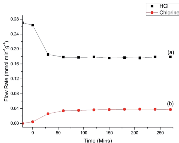
Fig. 7 (a) HCl and (b) Cl 2 flow rates observed for Deacon operation over the CuCl 2 /KCl/attapulgit catalyst as a function of time-on-stream at 653 K. Flow conditions: O 2 /He 20 cm 3 min -1 , HCl 6 cm 3 min -1 , N 2 (carrier gas) 33 cm 3 min -1 , and N 2 (diluent post-reactor) 100 cm 3 min -1 .
