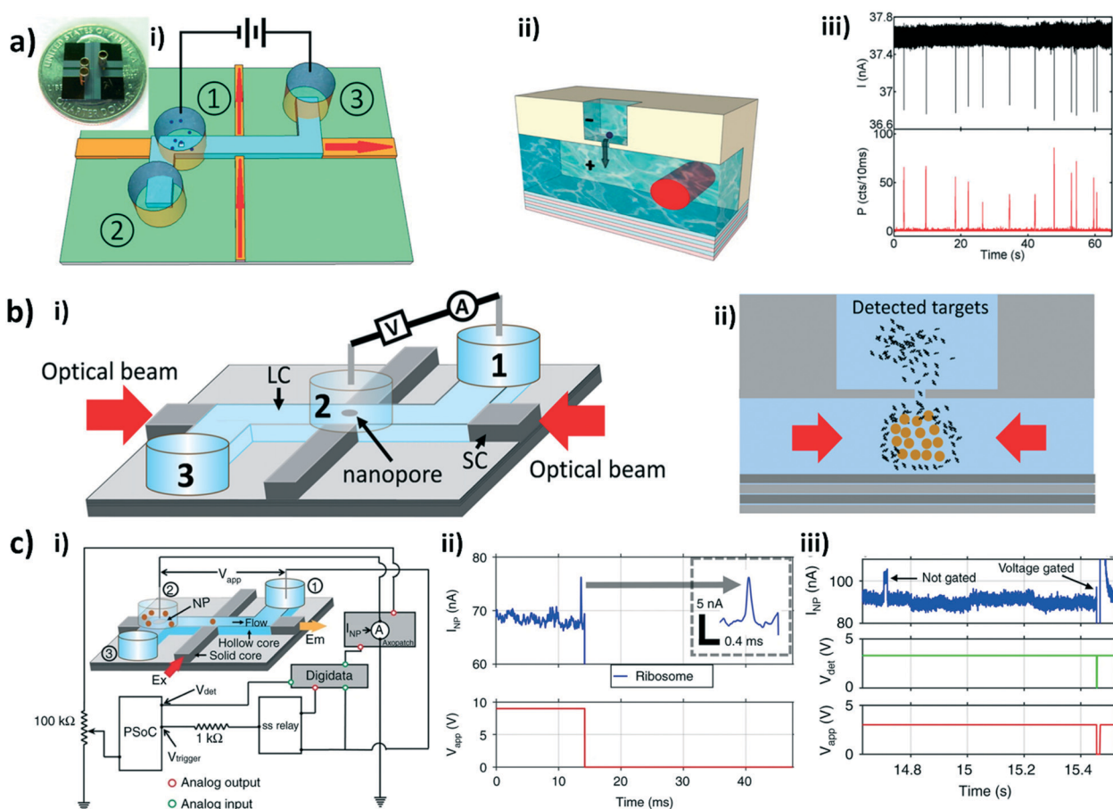
Fig. 8 Optofluidic integration with nanopore. a) Simultaneous electro-optical detection of single molecules in an optofluidic device. i) Schematic representation of the setup on an ARROW optofluidic device. ii) Cross-section of the nanopore and LC channel for visualization of the electro-optical detection methodology. iii) Actual electrical (black) and optical (red) trace of single H1N1 influenza virus detection. Reproduced with permission from ref. 52. b) Trap assisted capture rate enhancement of a nanopore. i) Schematic illustration of the experimental setup. ii) A cartoon depicting the conceptual visualization of TACRE. Reproduced with permission from ref. 95. c) On demand target delivery on a programmable ARROW optofluidic device. i) Schematic illustration with feedback control mechanism. ii) Current (top) and voltage (bottom) trace of a voltage gated single ribosome delivery. iii) Current (top), identification signal (middle) and voltage (bottom) trace of identification and voltage gating of only \lambda -DNAs from a mixture of \lambda -DNA and ribosome. Reproduced with permission from ref. 45.
