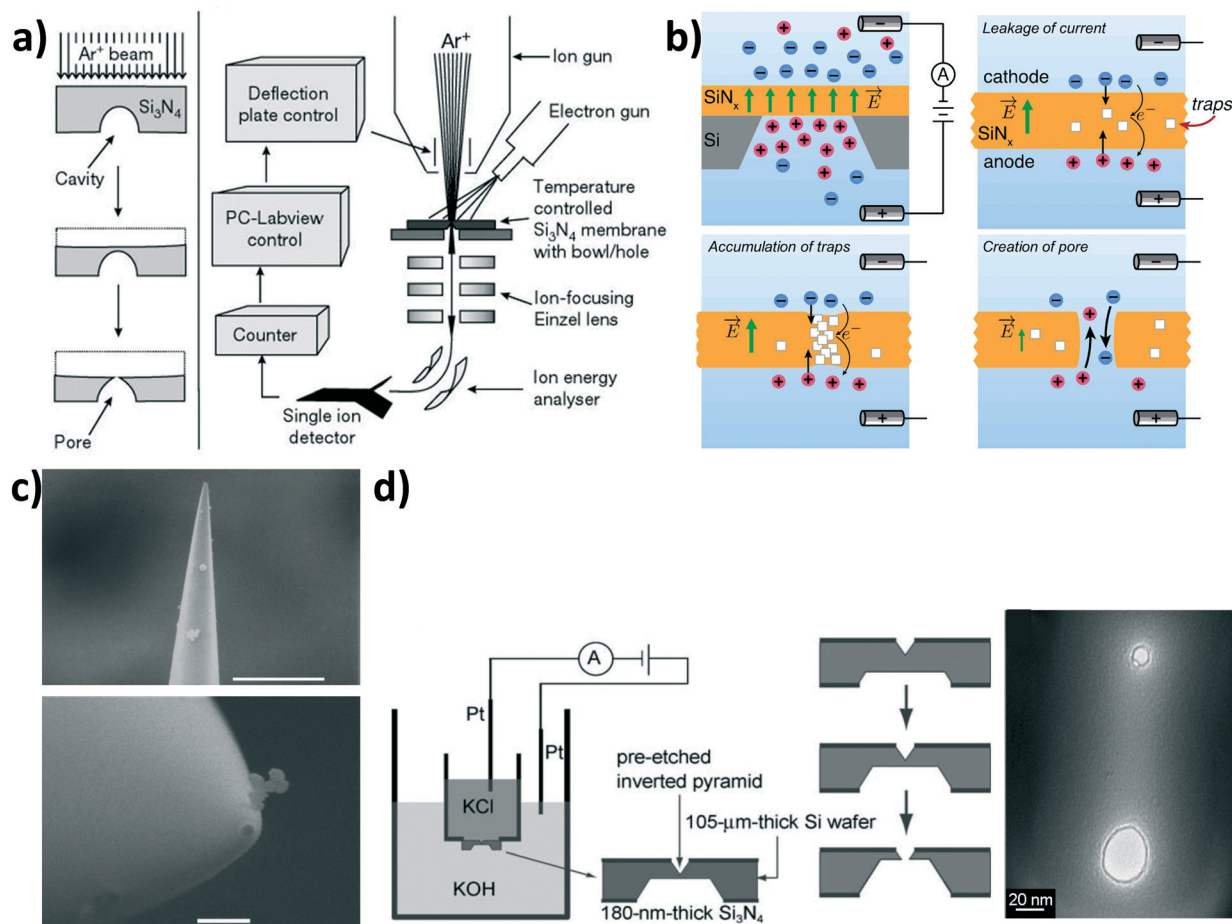
Fig. 2 Different nanopore fabrication techniques. a) Nanopore milling method using feedback-controlled ion beam sculping. Reproduced with permission from ref. 146. b) Step by step illustration of dielectric breakdown method for nanopore fabrication. Reproduced with permission from ref. 172. c) SEM images of a typical nanopipette (top) scale bar 2 \mu\text{m} and (bottom) 200 nm. Reproduced with permission from ref. 181. d) Schematic representation of experimental setup for nanopore fabrication using feedback controlled chemical etching. Reproduced with permission from ref. 187.
