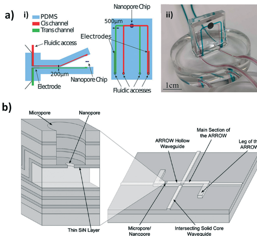
Fig. 3 Microfluidic integrated nanopore for electrical detection of target particles. a) Reusable nanopore device with microfluidic channels on PDMS. i) Schematic of cross sectional and top view of the device. ii) Photograph of a complete nanopore device with a nanopore chip clamped inside PDMS layers. Reproduced with permission from ref. 93. b) Schematic presentation of a typical ARROW optofluidic device with liquid channel and optical waveguides. Zoomed in image shows cross section view of the micropore and nanopore drilled on the liquid channel. Reproduced with permission from ref. 213.
