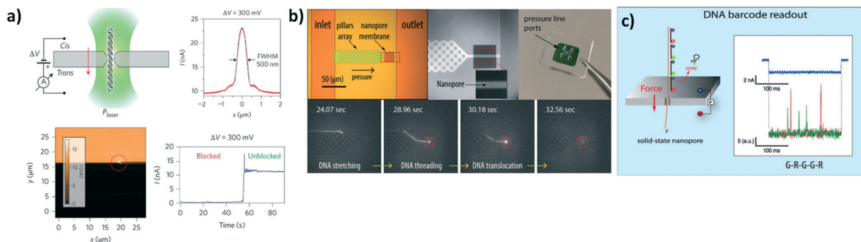
Fig. 5 Optical integration with nanopore. a) Optoelectronic control of nanopore surface charge. Top left: Schematic view of the optical integration with nanopore where a 532 nm wavelength laser beam is focused at the nanopore. This integration influences the translocation characteristics of a target particle. Top right: The ionic current profile with the position of the laser scan in x -axis. Bottom left: The two-dimensional ionic current profile of a clogged nanopore. Right after the laser scan passes the nanopore, it unclogs the nanopore and the nanopore current increases. Bottom right: The nanopore current change with time. The current jumps and stabilizes when the laser beam unclog the pore. Reproduced with permission from ref. 242. b) (Top figures) Bright field image of the device for on chip stretching, sorting and electro-optical detection of ultralong nucleic acid. (Bottom images) Time series photographs of stretching and translocation of optically tagged DNA molecule. Reproduced with permission from ref. 245. c) Schematic view of a two-colors (red and green) single fluorophores DNA barcode translocating through the nanopore. The recorded electrical and fluorescent signals show multimodal detection scheme. Reproduced with permission from ref. 248.
