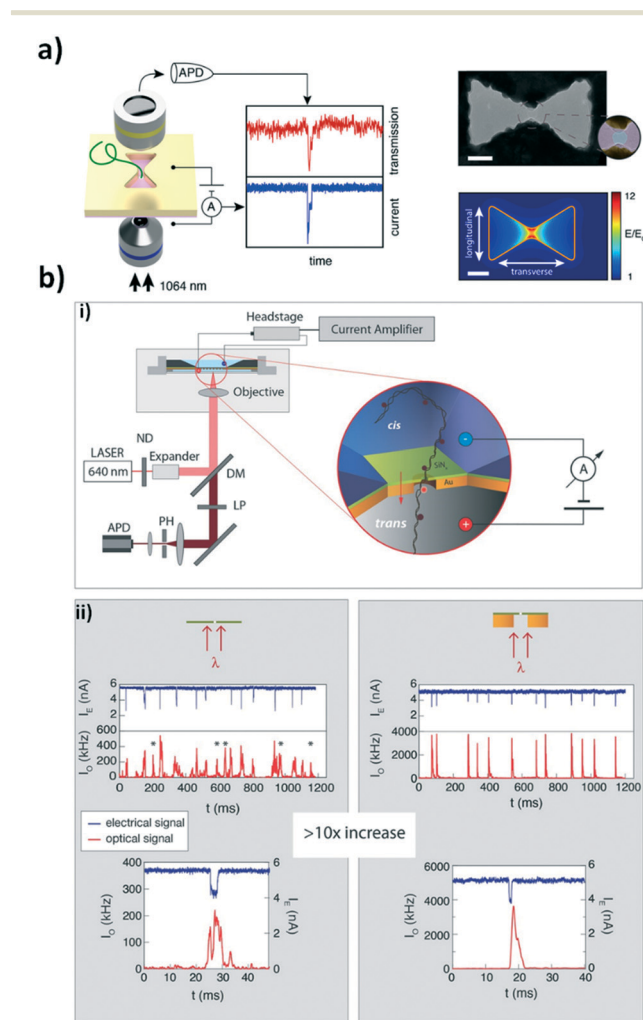
Fig. 7 Plasmonic nanopores. a) (Left) Schematic of inverted bowtie nanopore for label free particle detection. The optical transmission plot and nanopore current trace confirms simultaneous detection of a target particle. (Top right) TEM photograph of the inverted bow structure with a nanopore at the center. (Bottom right) Normalized electric field plot, simulated for the structure shown in the top right plot. Reproduced with permission from ref. 110. b) Simultaneous electro optical detection of labeled particle in a nanopore integrated plasmonic nano well (NP-PNW). i) Schematic of the experimental setup. ii) Comparison between electrical and optical signals obtained from standard nanopore device and NP-PNW device. Reproduced with permission from ref. 111.
