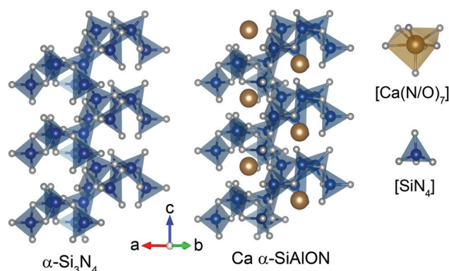
Fig. 1 Crystal structure of \alpha - \text{Si}_3\text{N}_4 and \text{Ca-}\alpha -SiAlON along c -axis. The brown, blue and gray spheres represent Ca, Si/Al, and N/O ions, respectively. The coordination polyhedron of Ca and Si tetrahedron are presented in right side.
