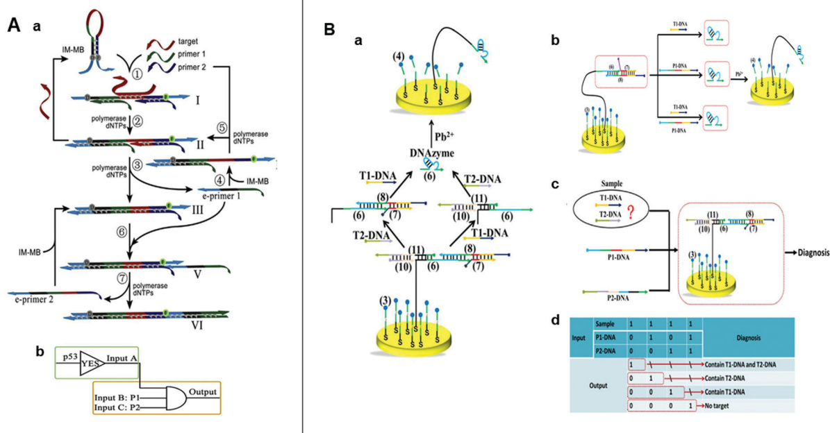
Fig. 5 (A) (a) Schematic illustration and (b) symbol of the SDA logic circuits. Reprinted from ref. 22, Copyright 2019, with permission from Elsevier. (B) (a) Schematic illustration of intelligent detection of T1-DNA and T2-DNA using DNA walker-based strategy. (b) Illustration of AND, (c) OR gate, (d) and the truth table for the combinatorial logic gates. Reprinted from ref. 23, Copyright 2018, with permission from Elsevier.
