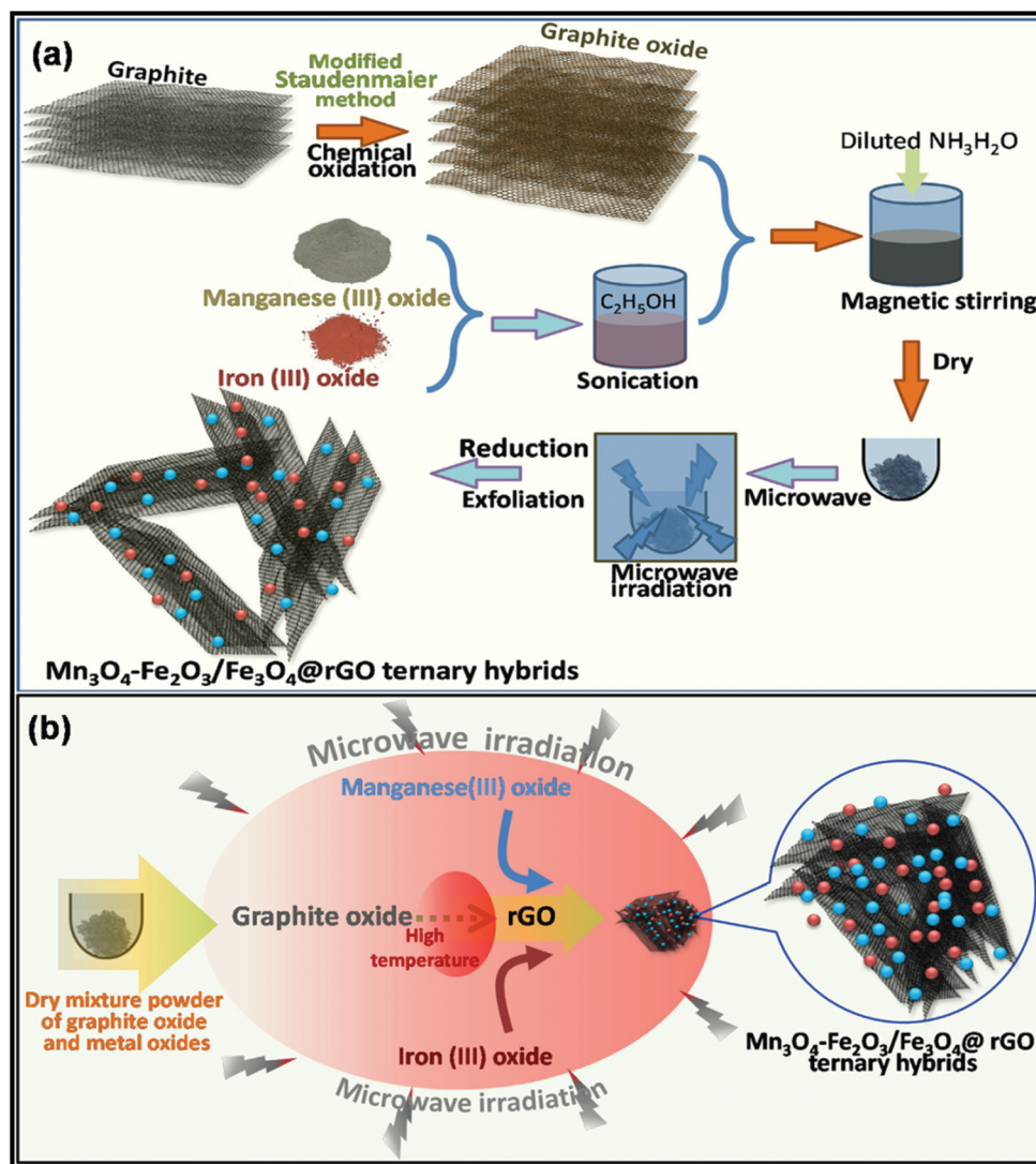
Fig. 13 Schematic presentation of the (a) synthesis process and (b) mechanism of MW-assisted formation of Mn_3O_4-Fe_2O_3/Fe_3O_4@rGO ternary hybrid. 222 Reprinted (adapted) with permission from ref. 222, copyright (2020), Elsevier B.V. All rights reserved.
