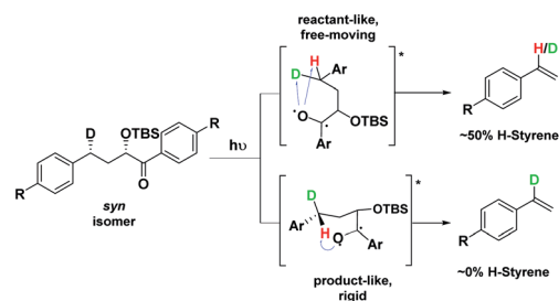
Scheme 2 Photolysis of the syn isomer gives between 0–50% H-styrene.
