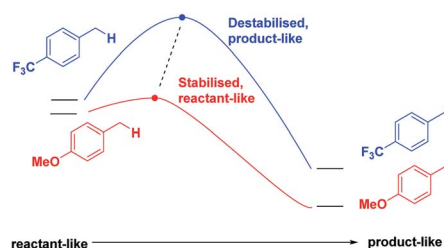
Fig. 6 Electronic effects on the ESTS.
