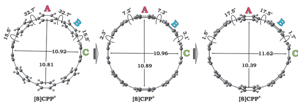
Fig. 5 Optimized geometries along with selected geometrical parameters for \text{1}^0 , \text{1}^{2-} , and \text{1}^{4-} (PBE0/cc-pVTZ).
